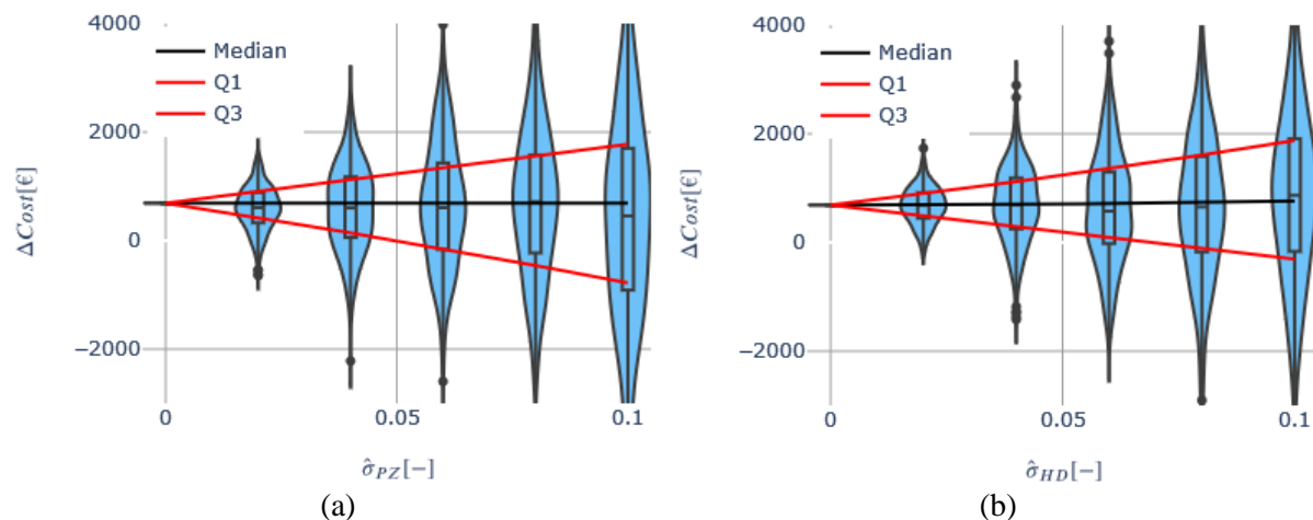
Figure 6: electricity price (a) and heat demand (b) uncertainty impact on actual costs
