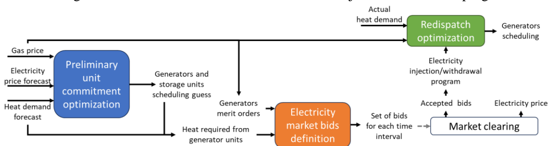
Figure 4: Three-stage optimization including the definition and submission of an optimal set of bids.
